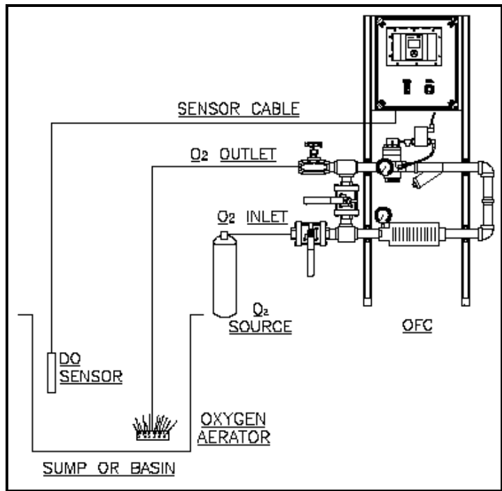
SYSTEM DIAGRAM
