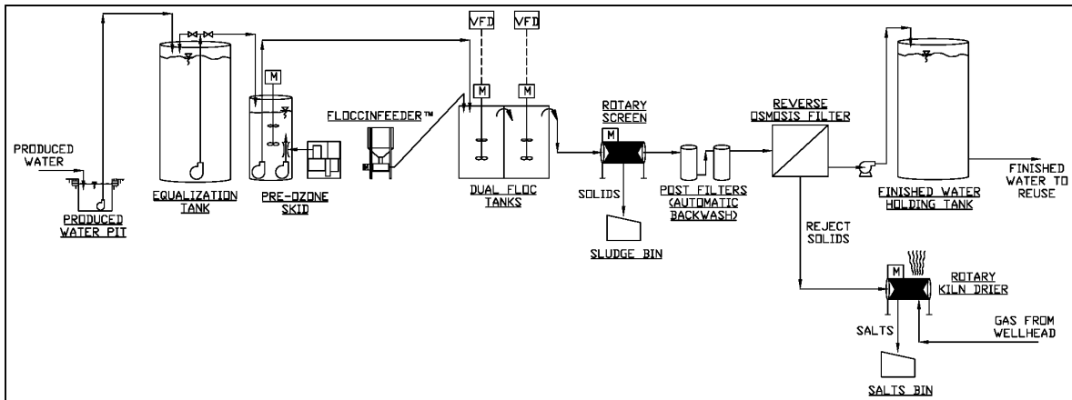
OFTS Process Diagram
